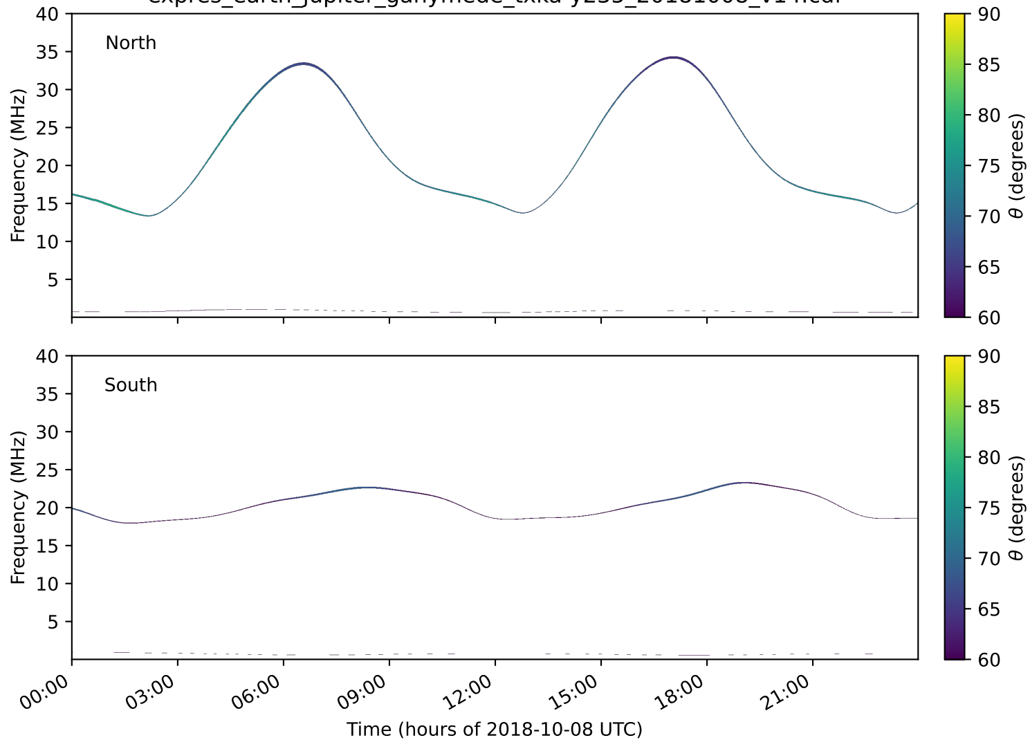
expres_earth_jupiter_ganymede_txka-y235_20181008_v14.cdf
