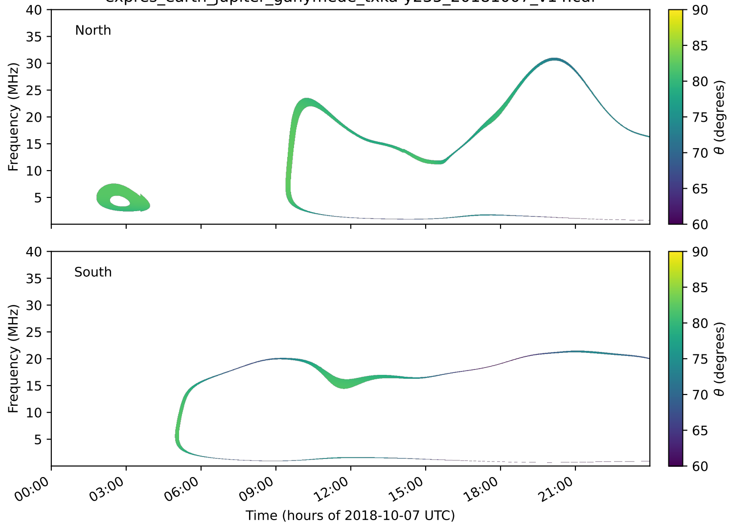
expres_earth_jupiter_ganymede_txka-y235_20181007_v14.cdf
