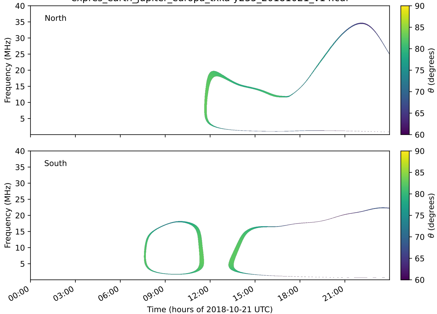
expres_earth_jupiter_europa_txka-y235_20181021_v14.cdf
