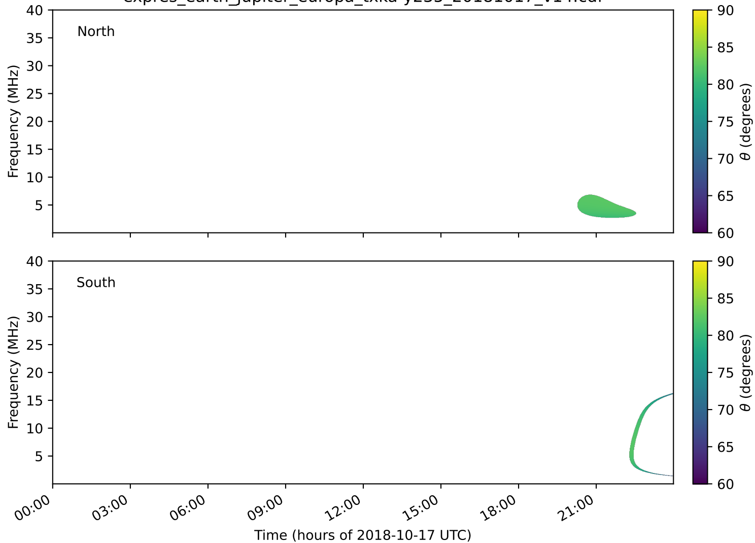
expres_earth_jupiter_europa_txka-y235_20181017_v14.cdf
