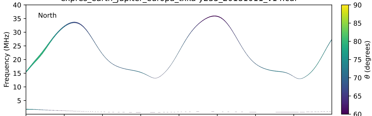
expres_earth_jupiter_europa_txka-y235_20181011_v14.cdf
