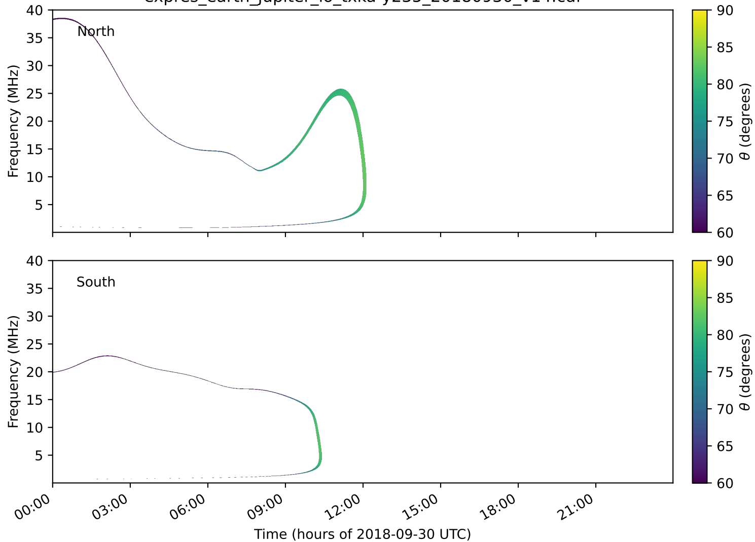
expres_earth_jupiter_io_txka-y235_20180930_v14.cdf
