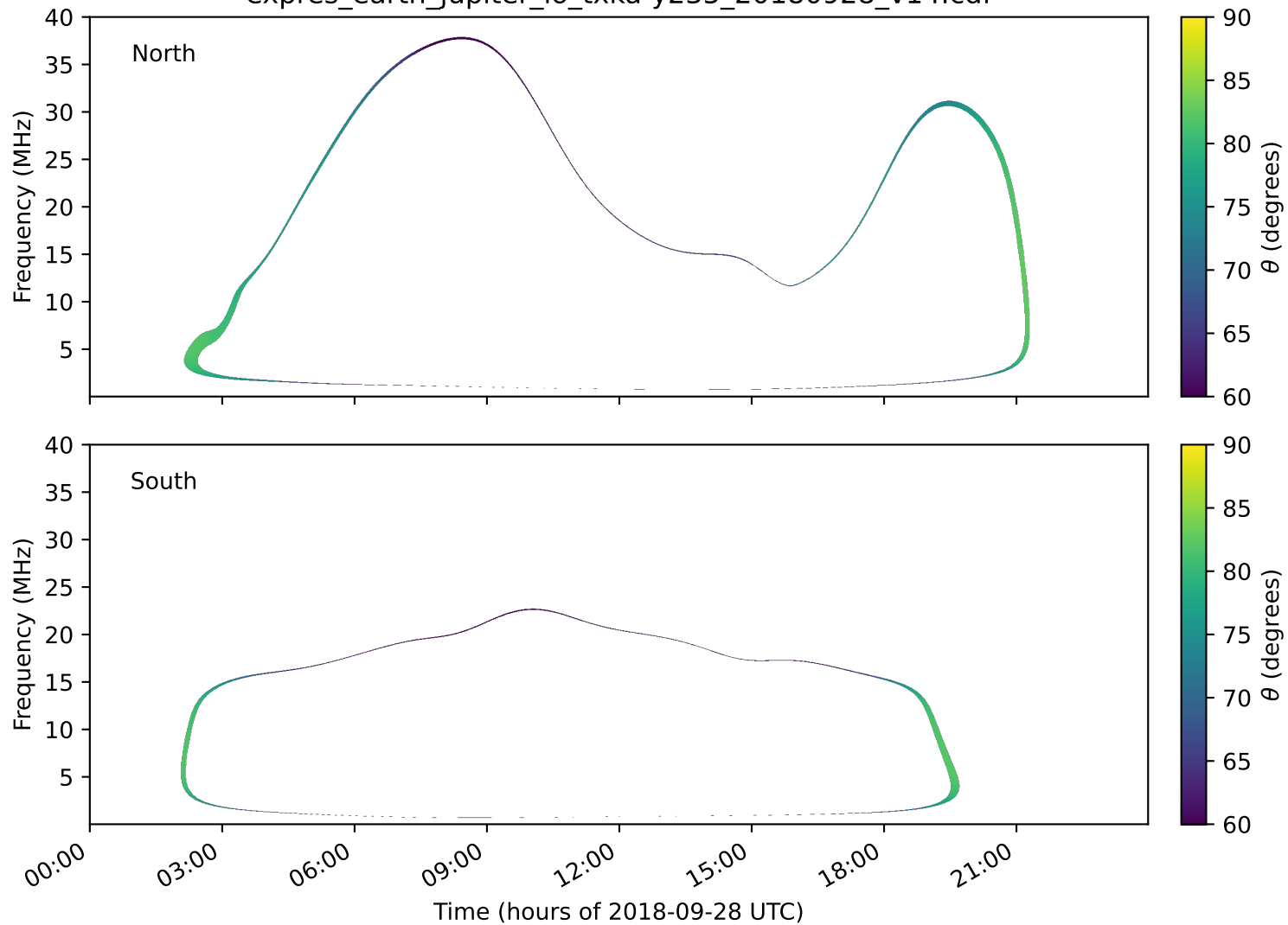
expres_earth_jupiter_io_txka-y235_20180928_v14.cdf
