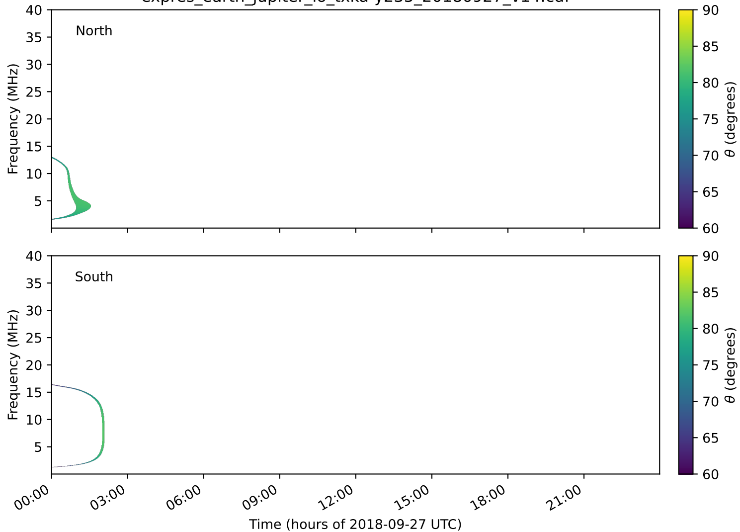
expres_earth_jupiter_io_txka-y235_20180927_v14.cdf
