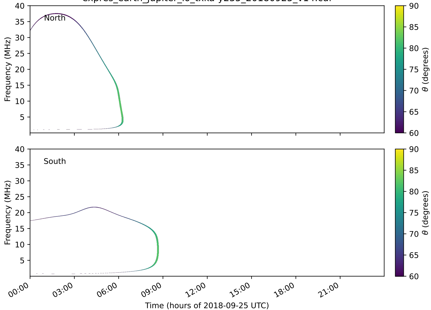
expres_earth_jupiter_io_txka-y235_20180925_v14.cdf
