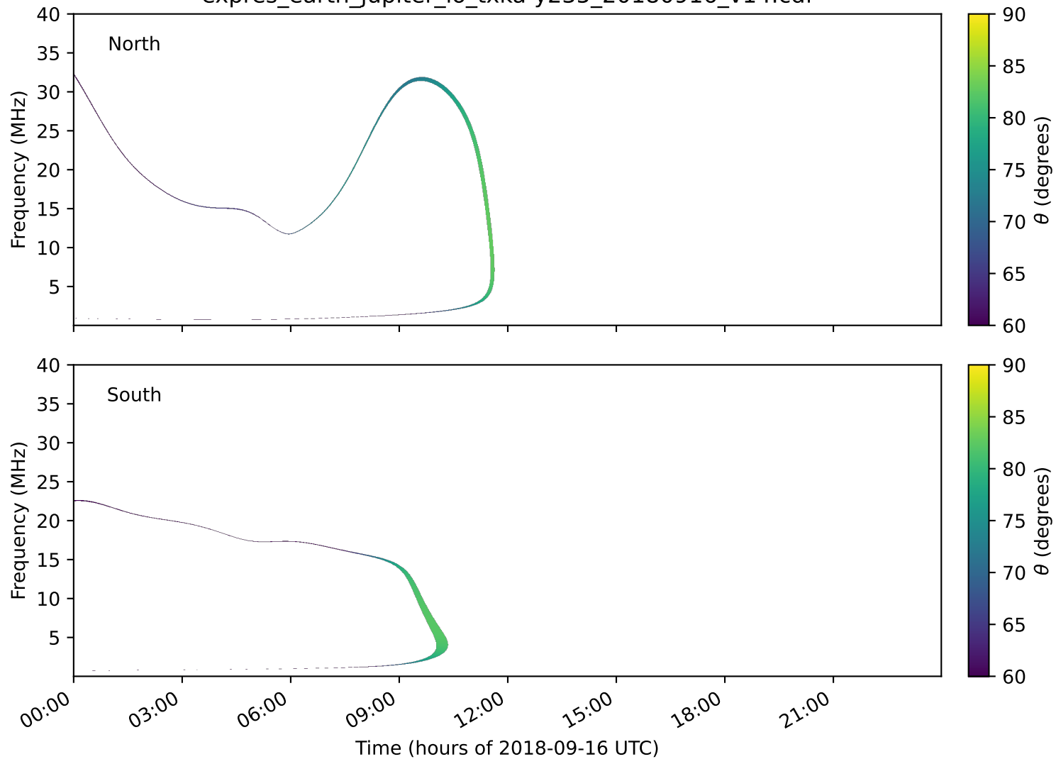
expres_earth_jupiter_io_txka-y235_20180916_v14.cdf
