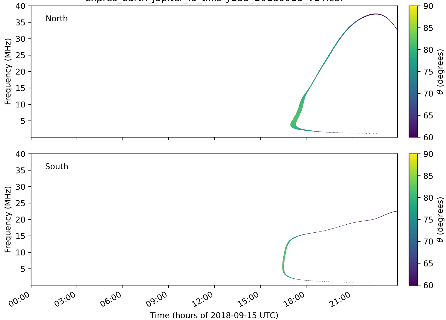
expres_earth_jupiter_io_txka-y235_20180915_v14.cdf
