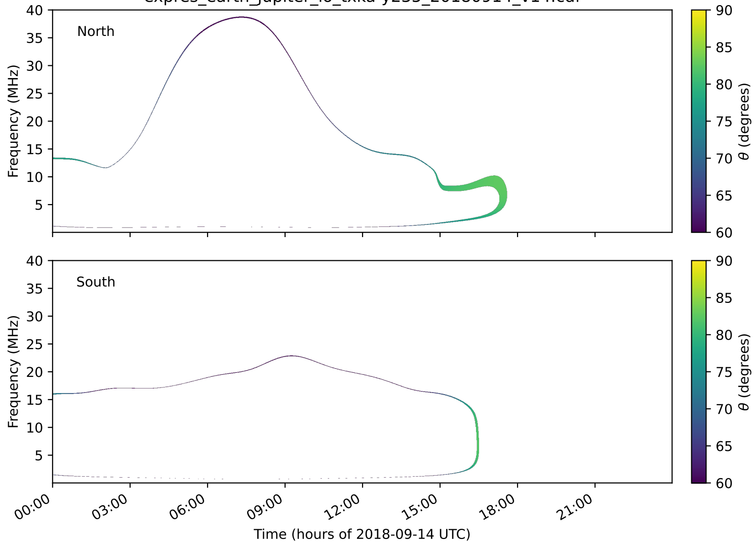
expres_earth_jupiter_io_txka-y235_20180914_v14.cdf
