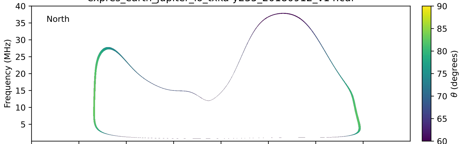
expres_earth_jupiter_io_txka-y235_20180912_v14.cdf
