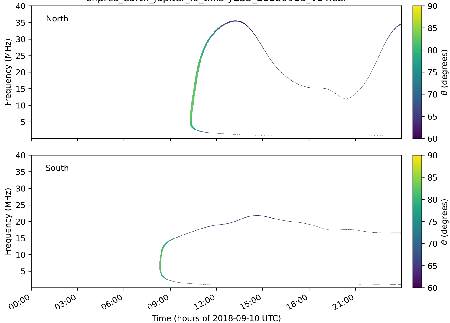
expres_earth_jupiter_io_txka-y235_20180910_v14.cdf
