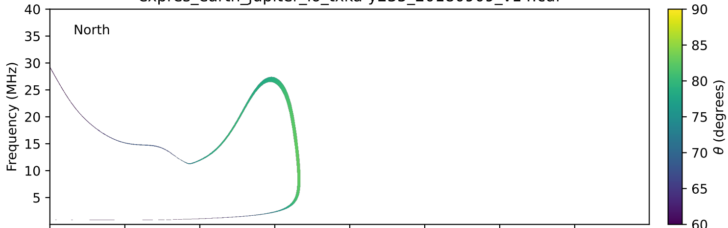
expres_earth_jupiter_io_txka-y235_20180909_v14.cdf
