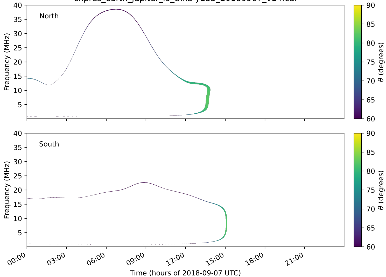
expres_earth_jupiter_io_txka-y235_20180907_v14.cdf
