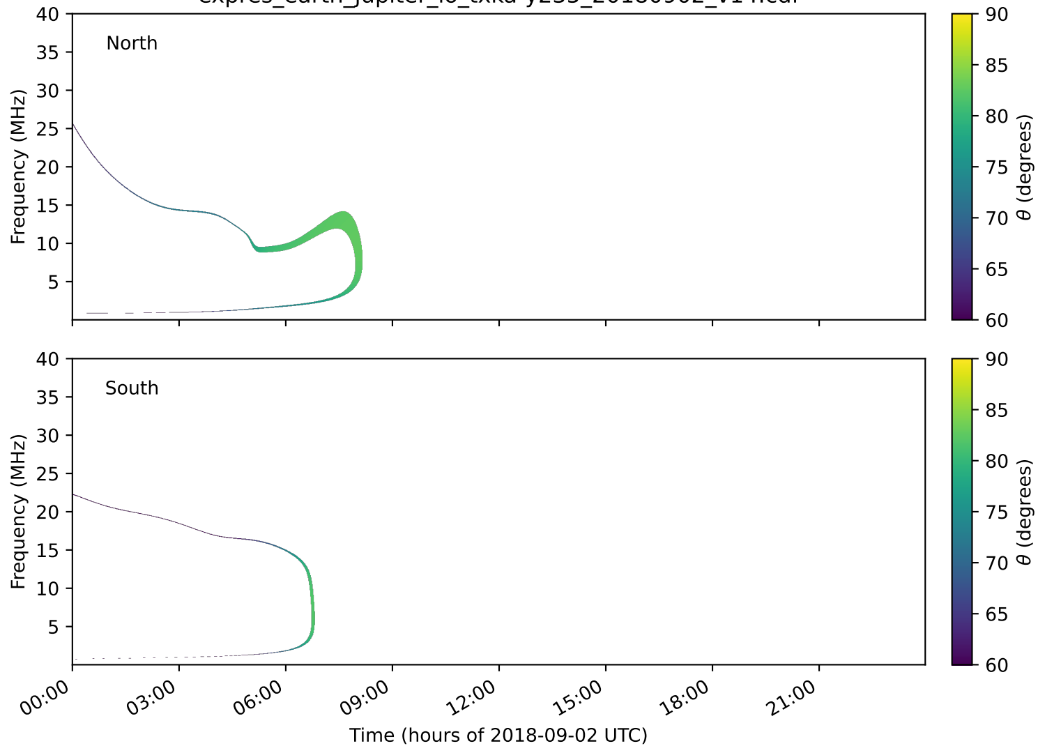
expres_earth_jupiter_io_txka-y235_20180902_v14.cdf
