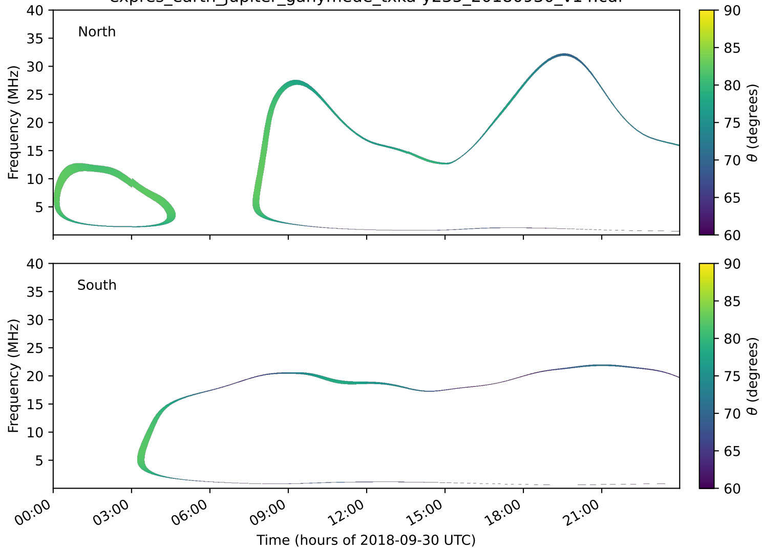
expres_earth_jupiter_ganymede_txka-y235_20180930_v14.cdf
