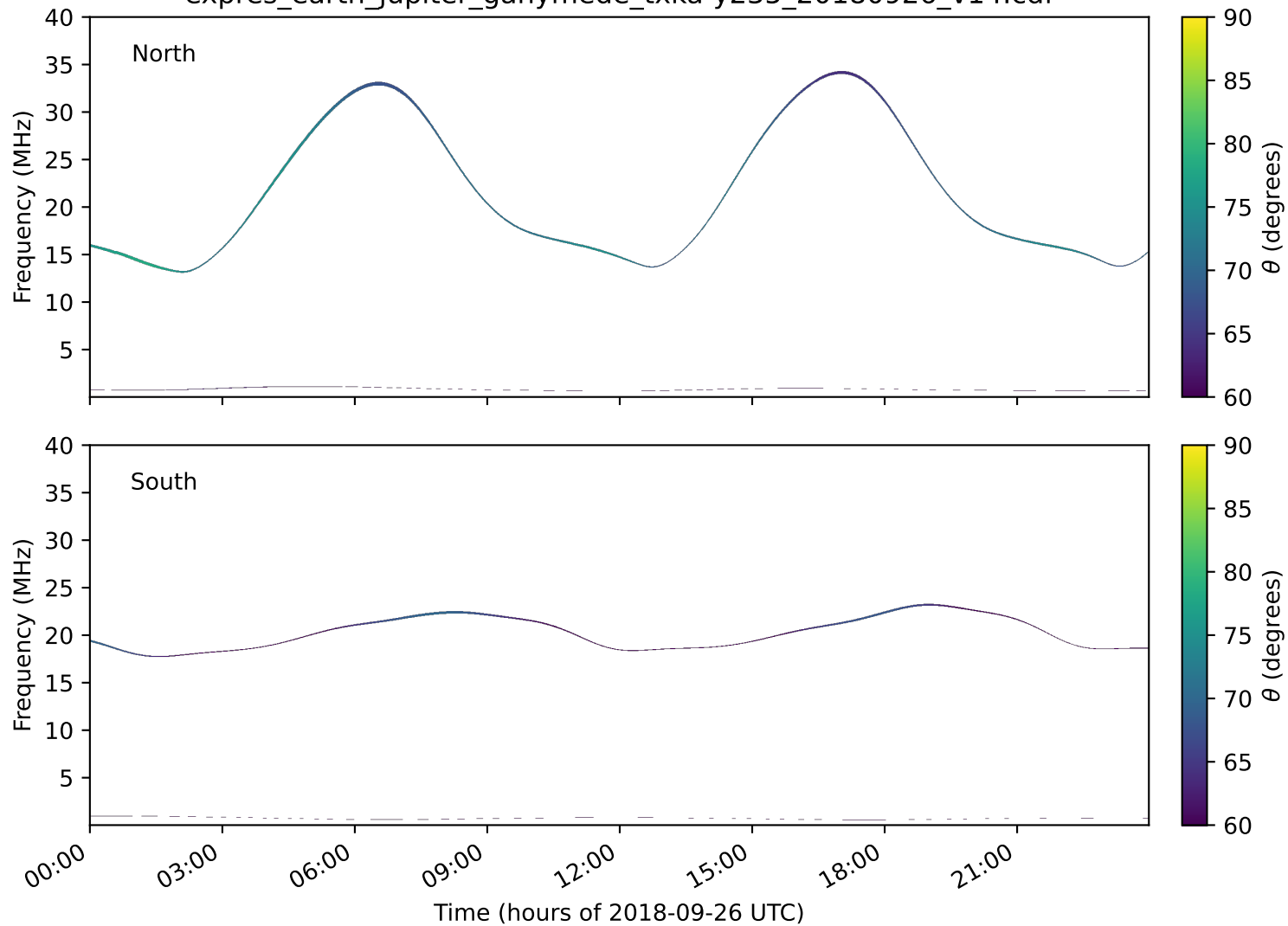
expres_earth_jupiter_ganymede_txka-y235_20180926_v14.cdf
