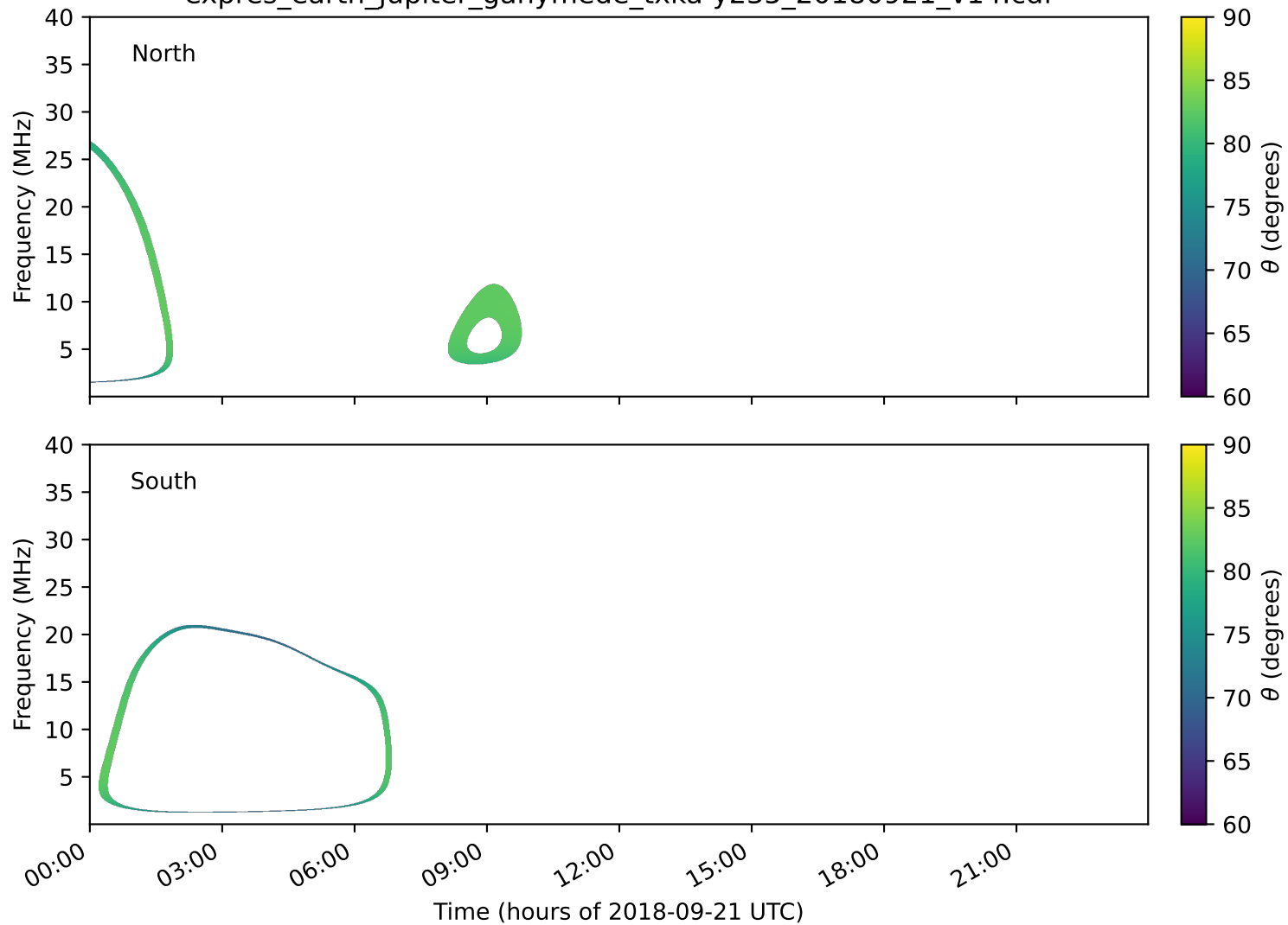
expres_earth_jupiter_ganymede_txka-y235_20180921_v14.cdf
