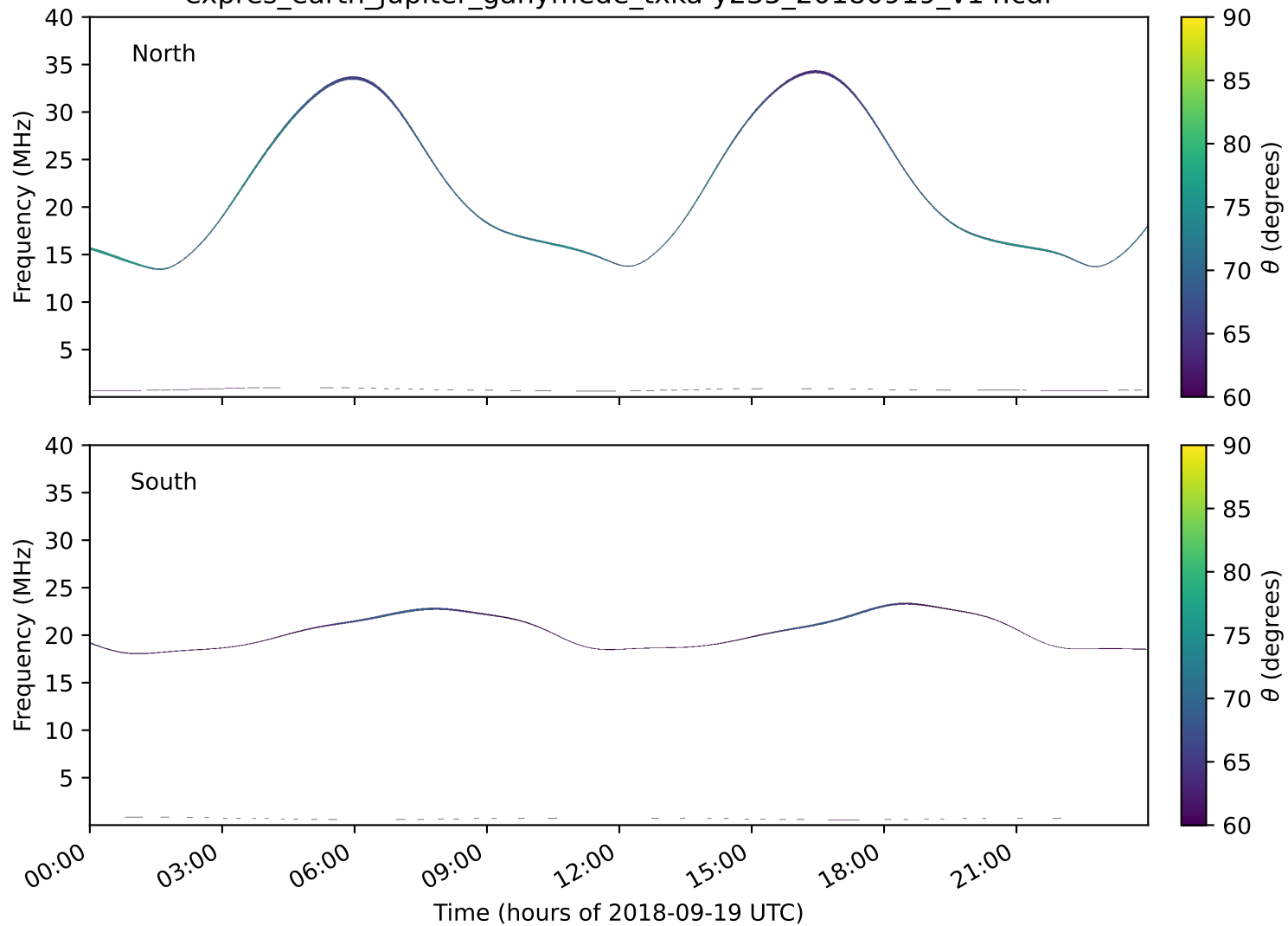
expres_earth_jupiter_ganymede_txka-y235_20180919_v14.cdf
