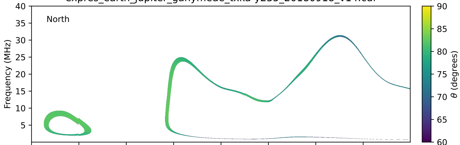
expres_earth_jupiter_ganymede_txka-y235_20180918_v14.cdf
