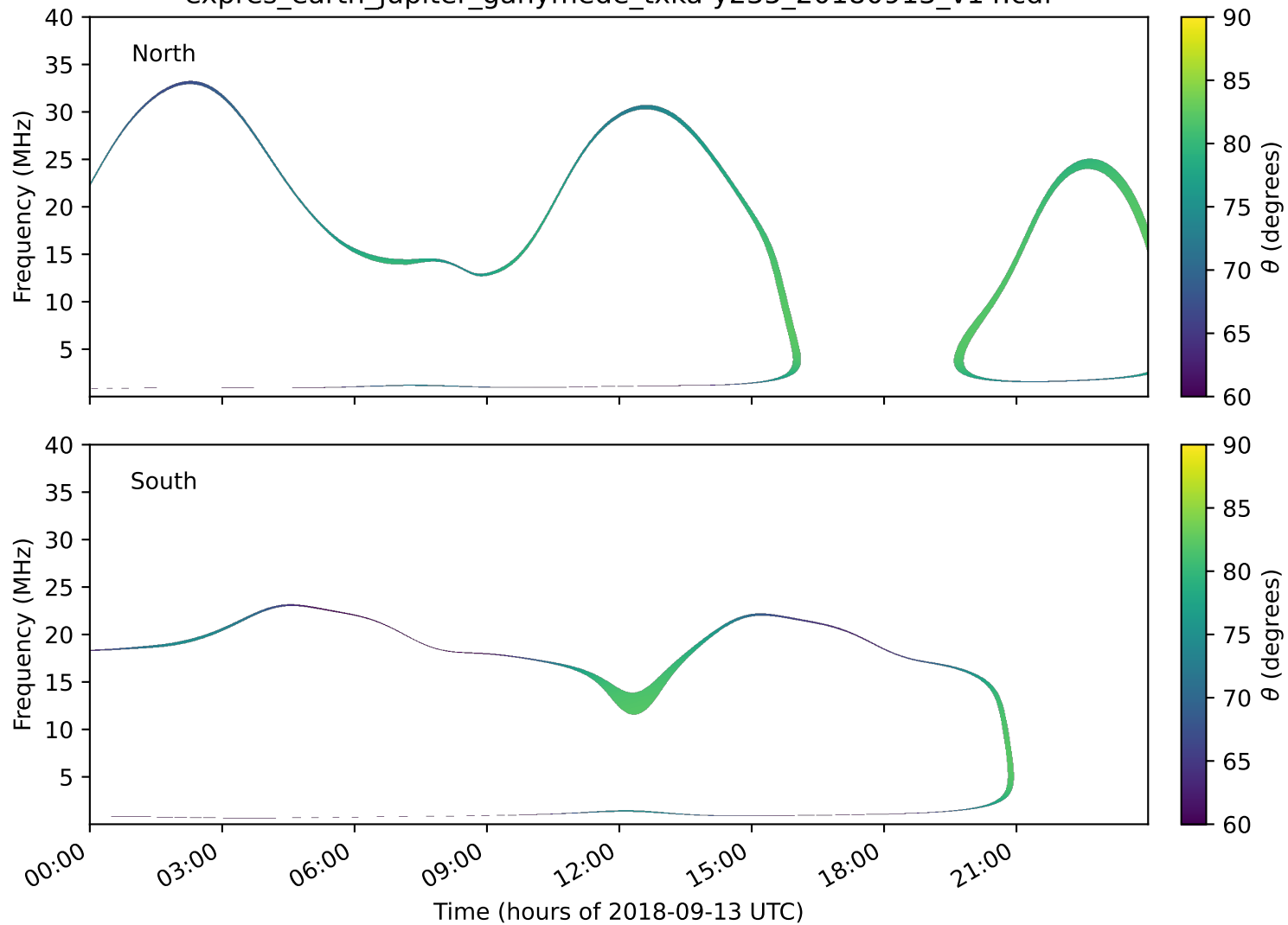
expres_earth_jupiter_ganymede_txka-y235_20180913_v14.cdf
