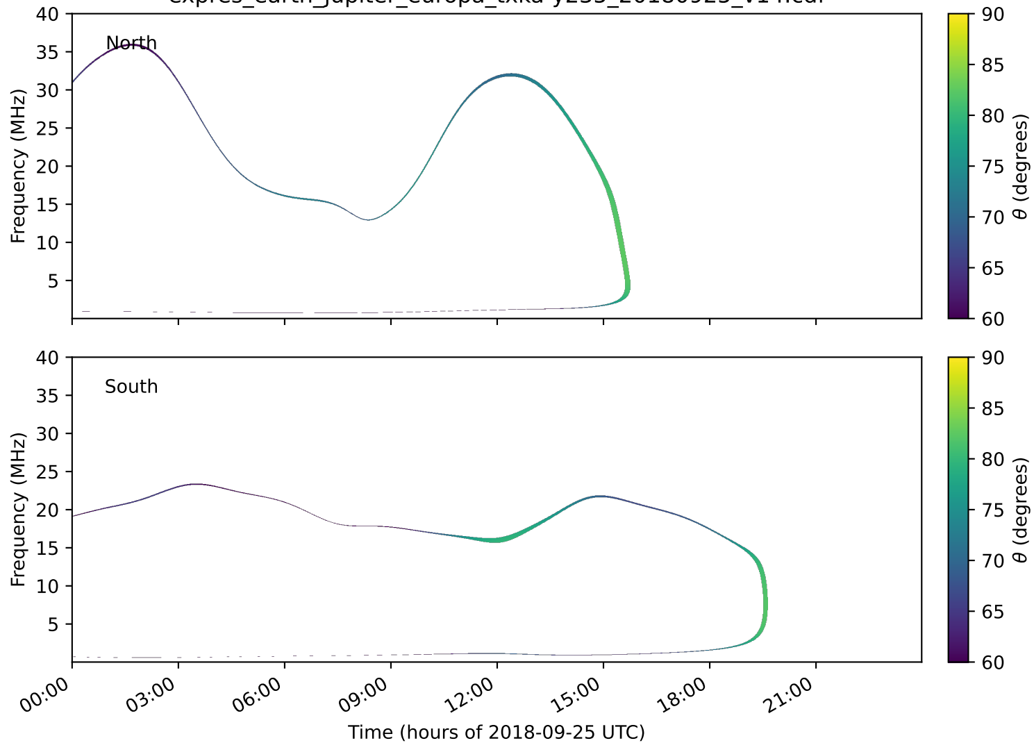
expres_earth_jupiter_europa_txka-y235_20180925_v14.cdf
