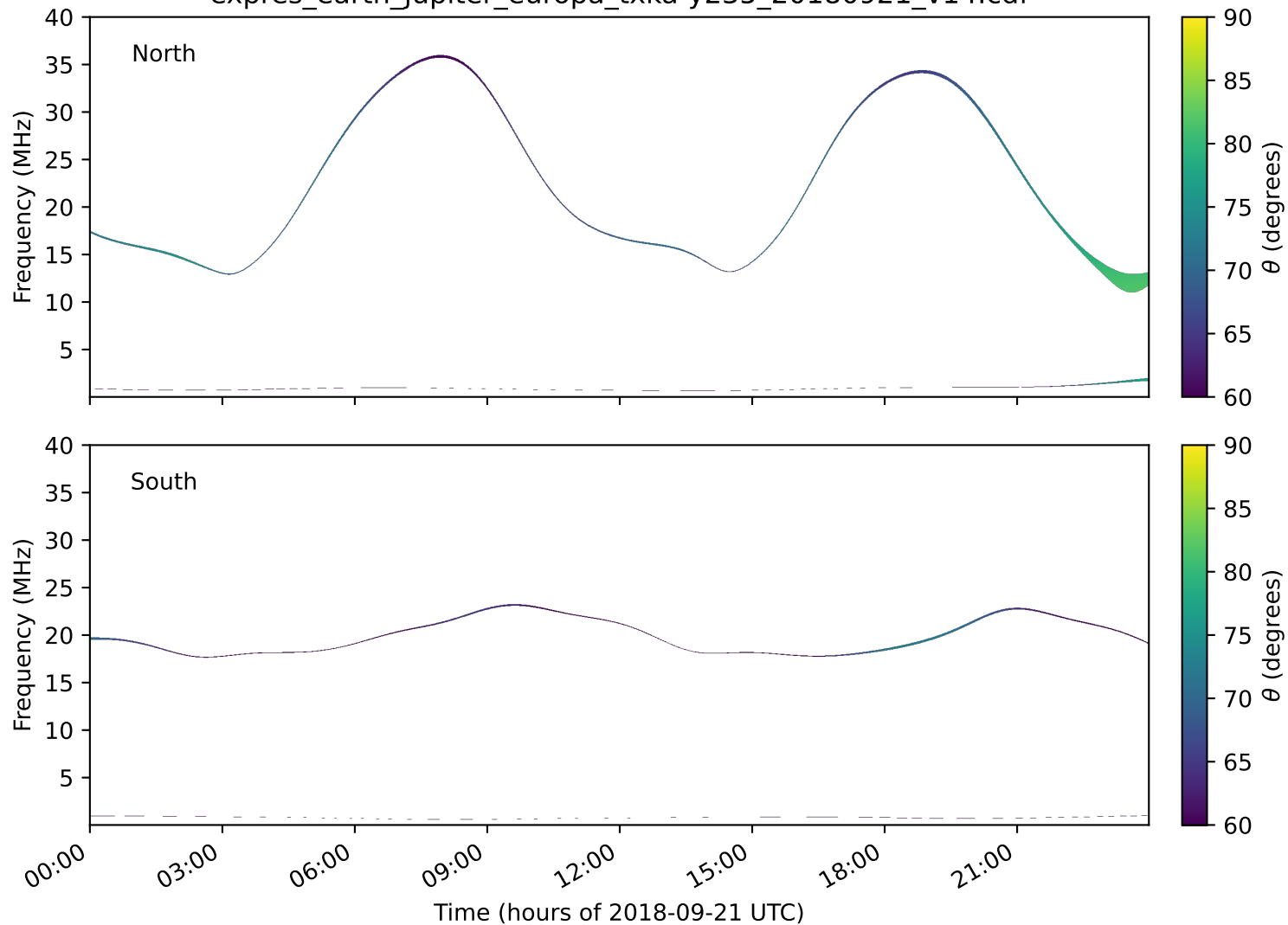
expres_earth_jupiter_europa_txka-y235_20180921_v14.cdf
