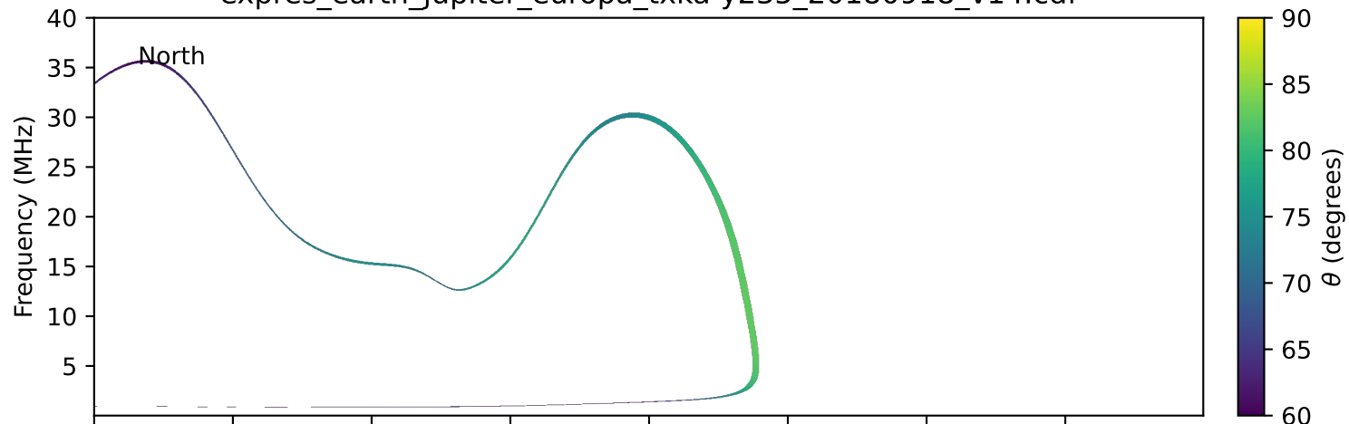
expres_earth_jupiter_europa_txka-y235_20180918_v14.cdf
