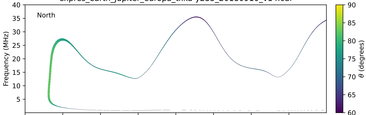
expres_earth_jupiter_europa_txka-y235_20180910_v14.cdf
