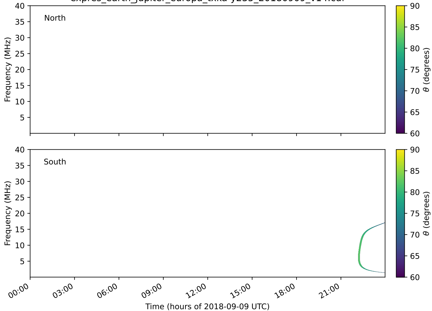
expres_earth_jupiter_europa_txka-y235_20180909_v14.cdf
