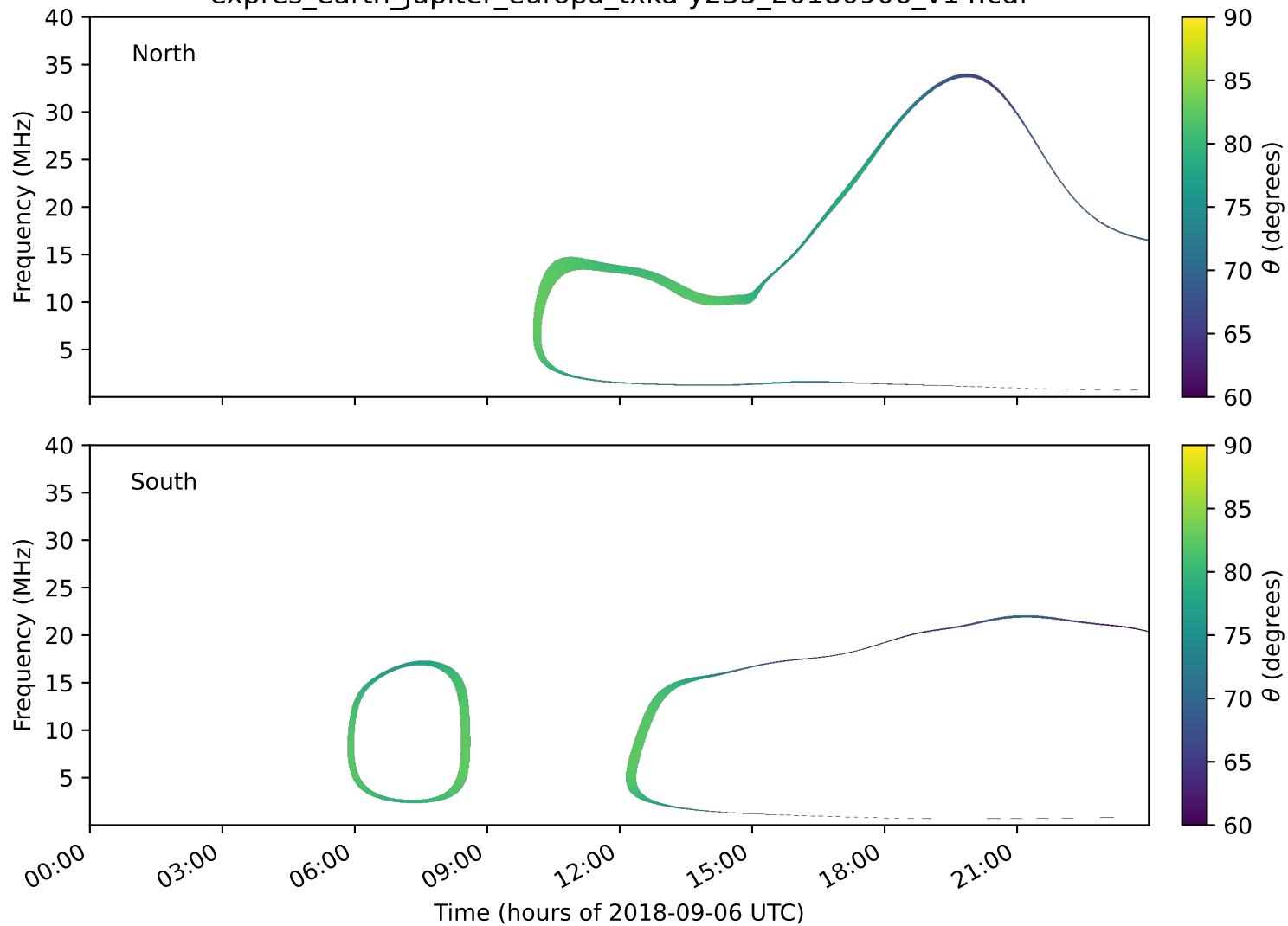
expres_earth_jupiter_europa_txka-y235_20180906_v14.cdf
