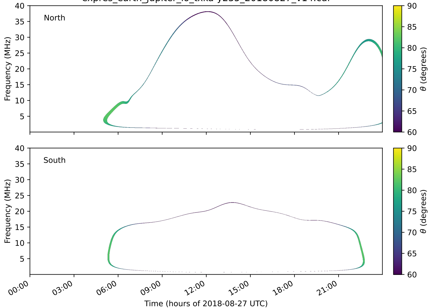
expres_earth_jupiter_io_txka-y235_20180827_v14.cdf
