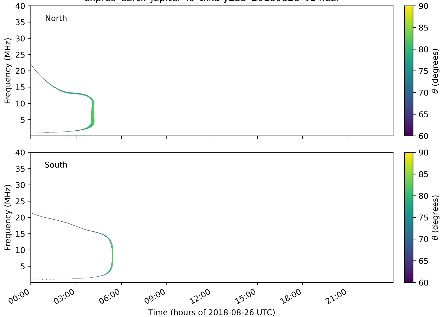
expres_earth_jupiter_io_txka-y235_20180826_v14.cdf
