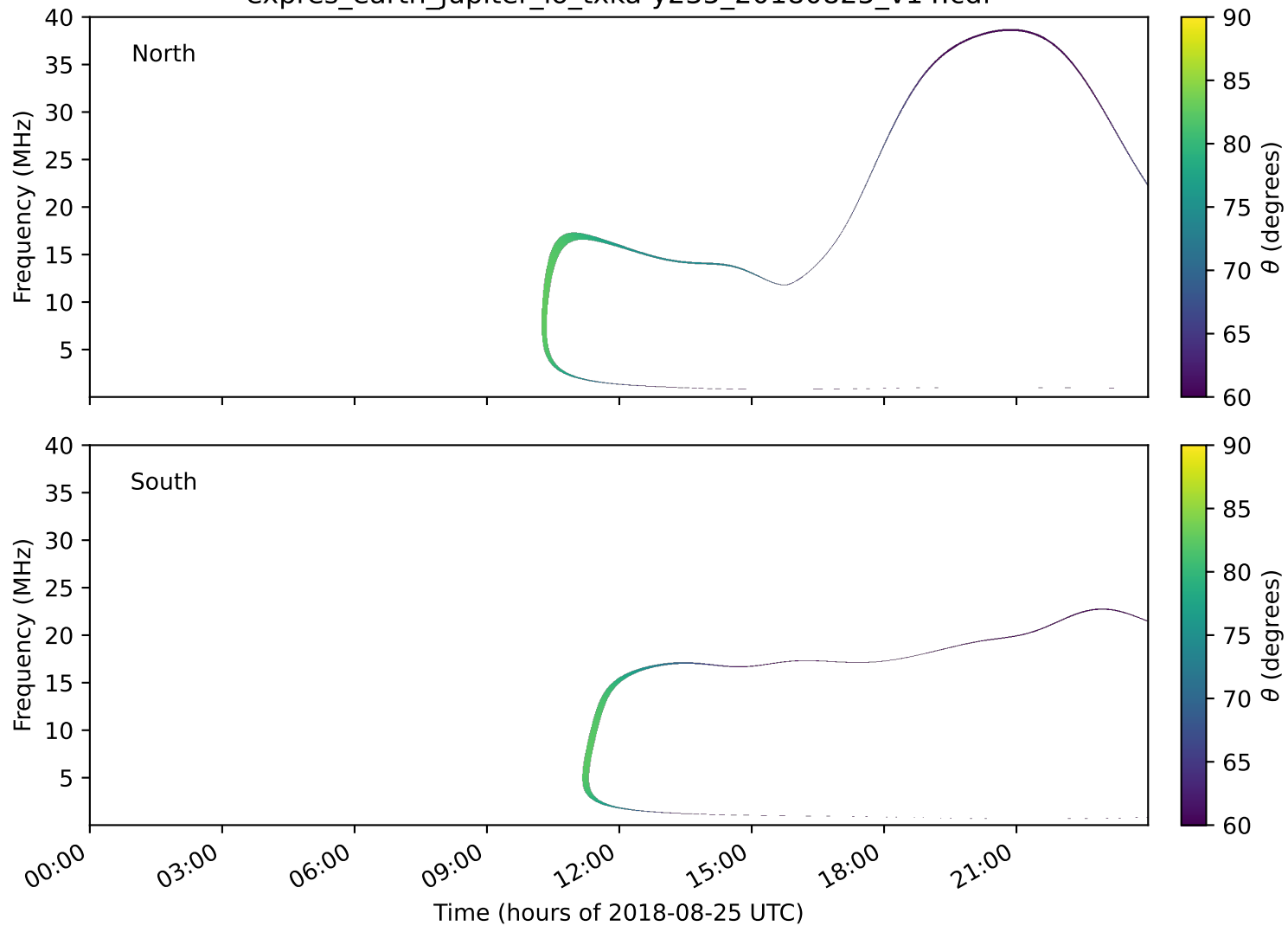
expres_earth_jupiter_io_txka-y235_20180825_v14.cdf
