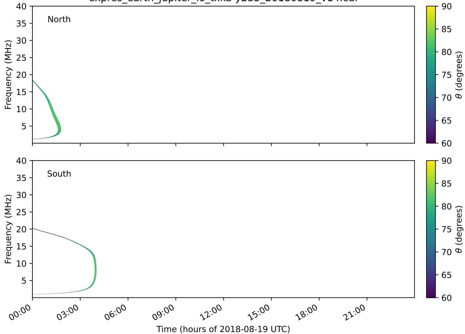
expres_earth_jupiter_io_txka-y235_20180819_v14.cdf
