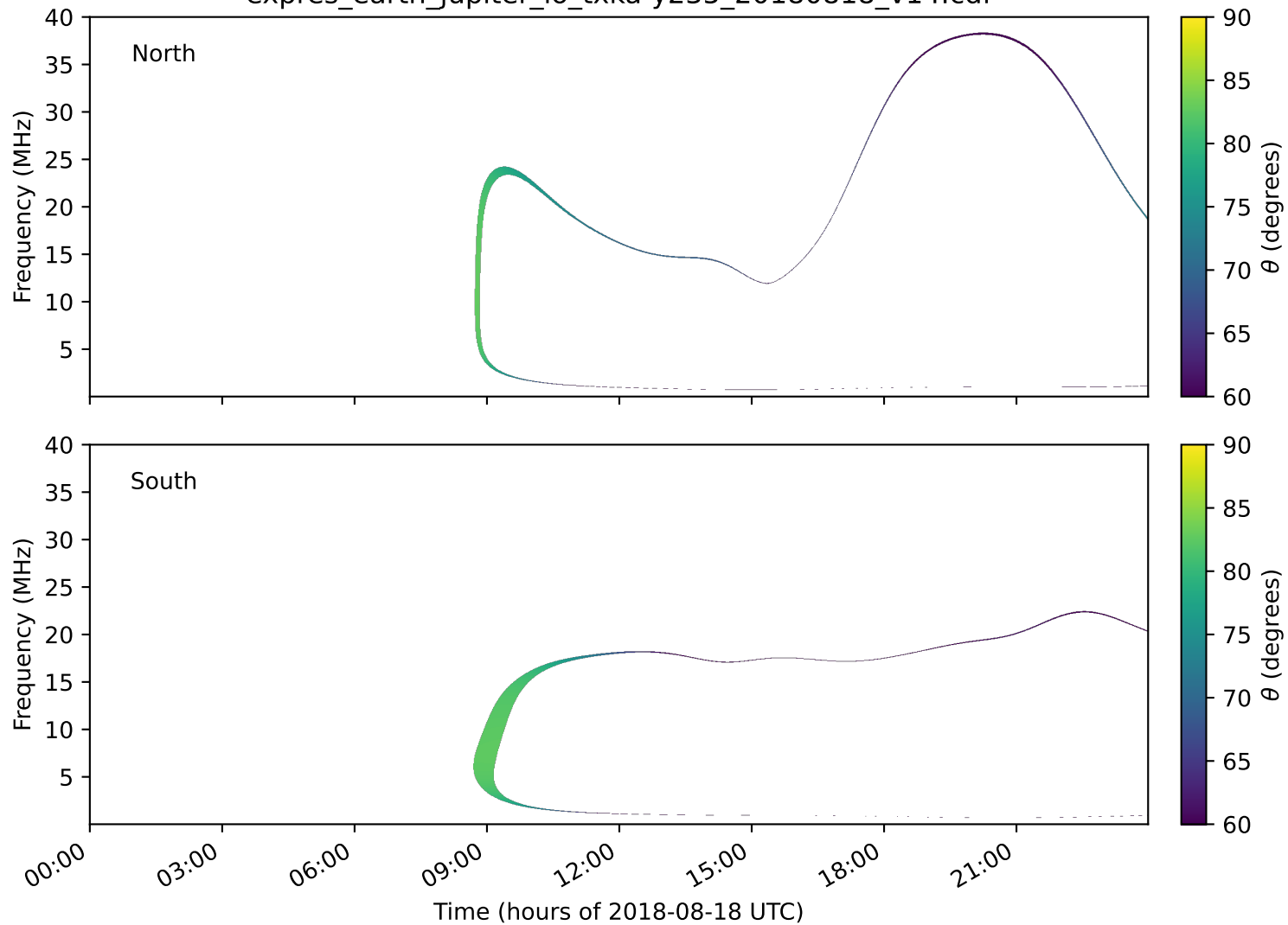
expres_earth_jupiter_io_txka-y235_20180818_v14.cdf
