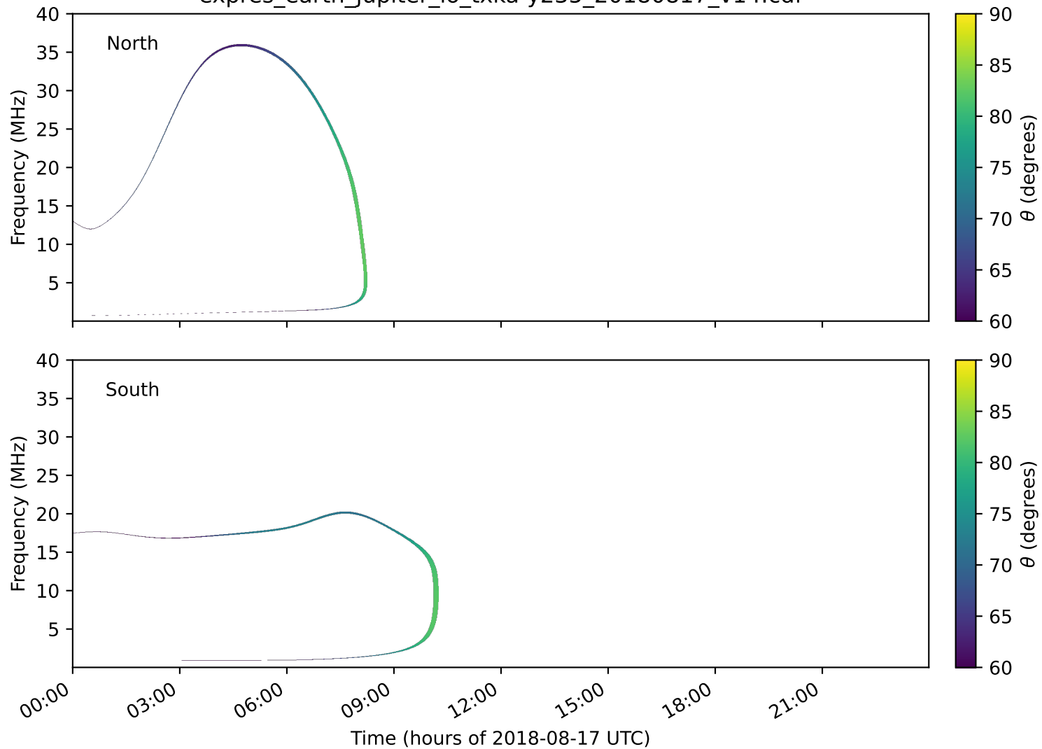
expres_earth_jupiter_io_txka-y235_20180817_v14.cdf
