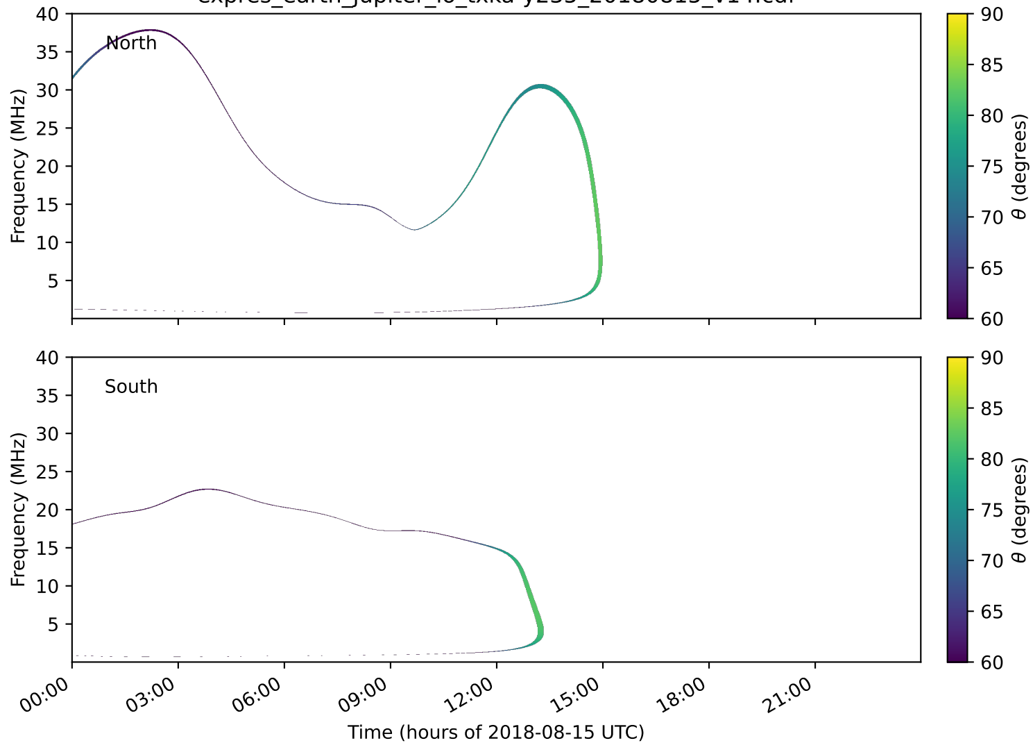
expres_earth_jupiter_io_txka-y235_20180815_v14.cdf
