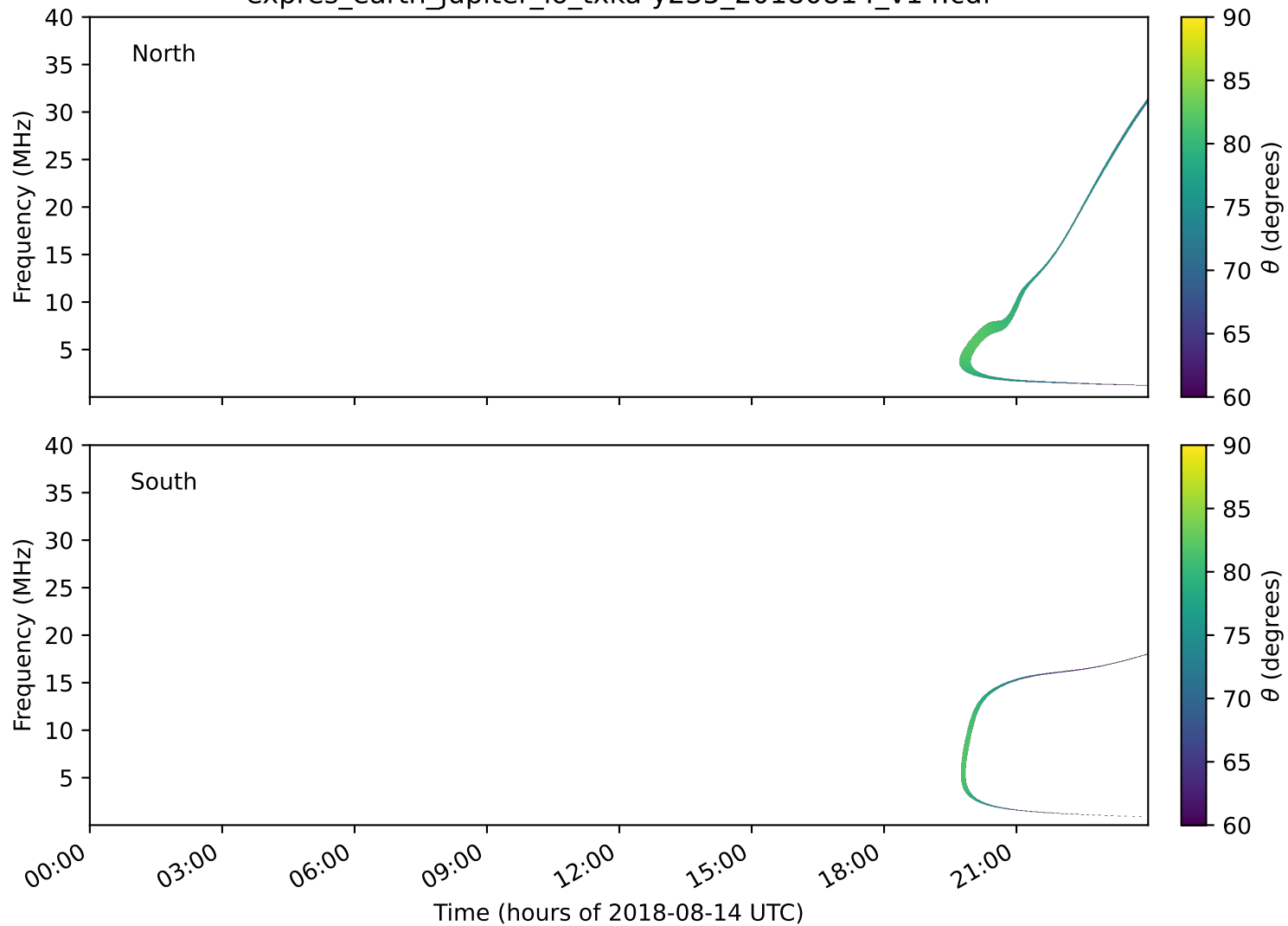
expres_earth_jupiter_io_txka-y235_20180814_v14.cdf
