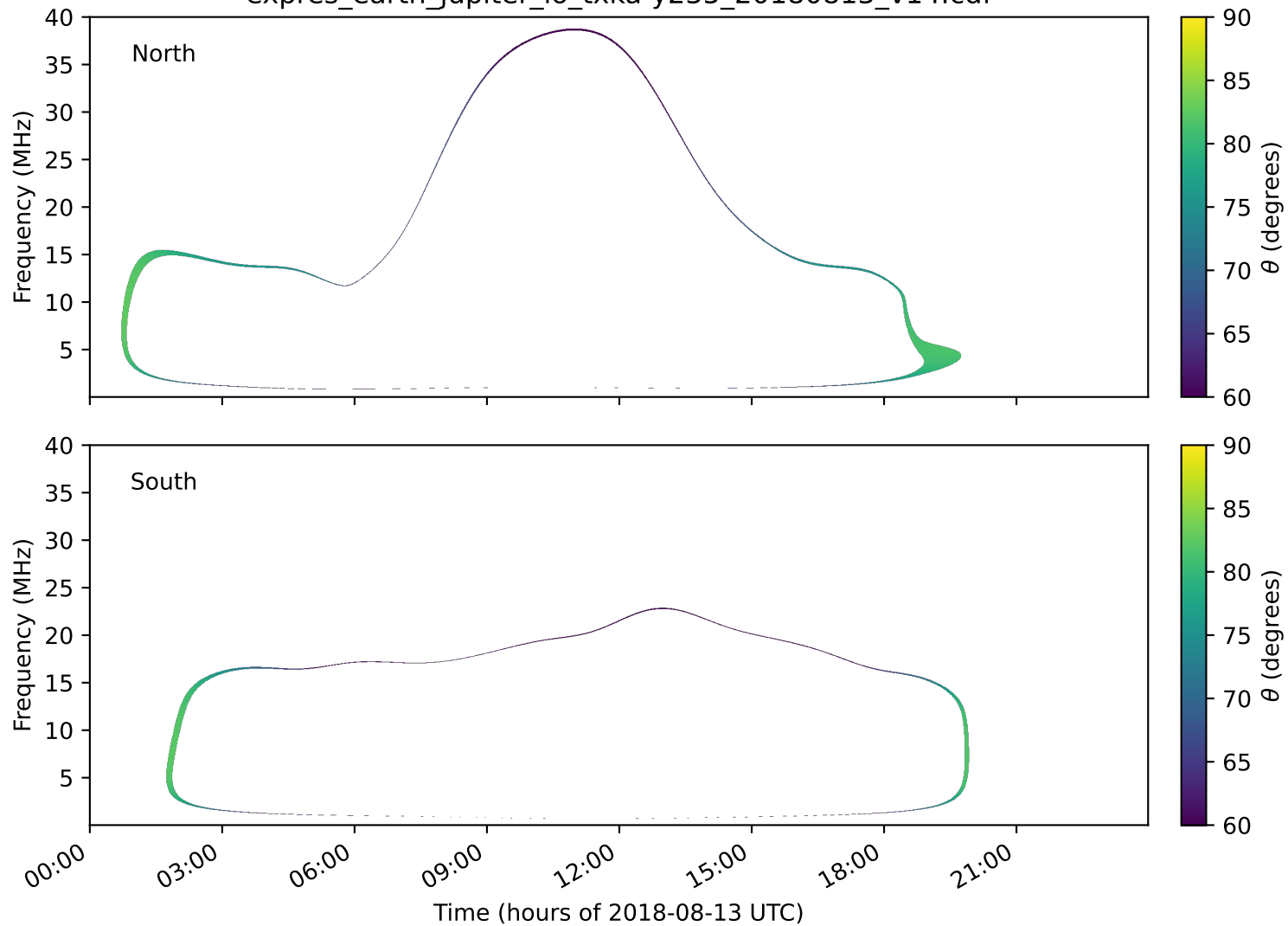
expres_earth_jupiter_io_txka-y235_20180813_v14.cdf
