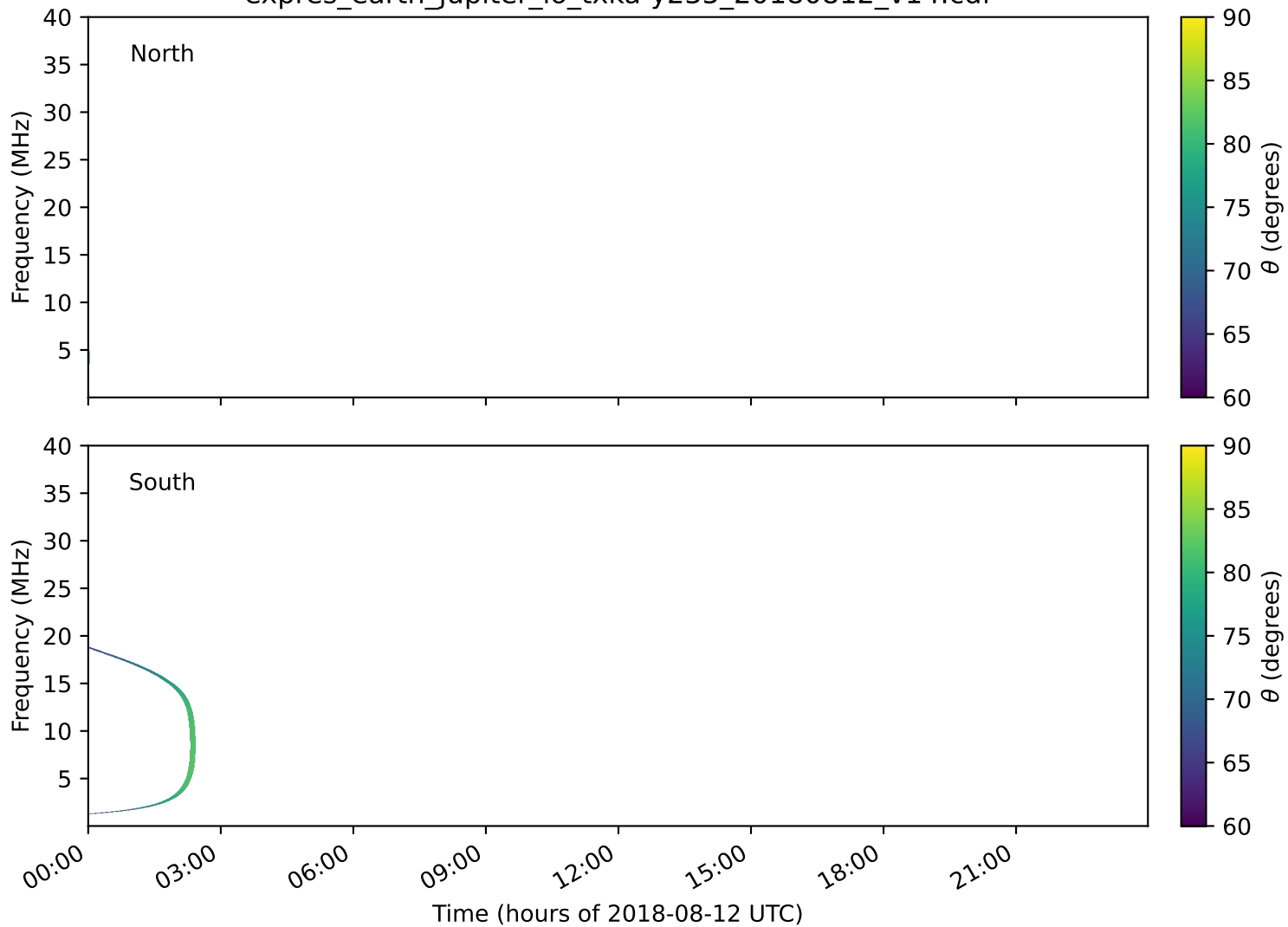
expres_earth_jupiter_io_txka-y235_20180812_v14.cdf
