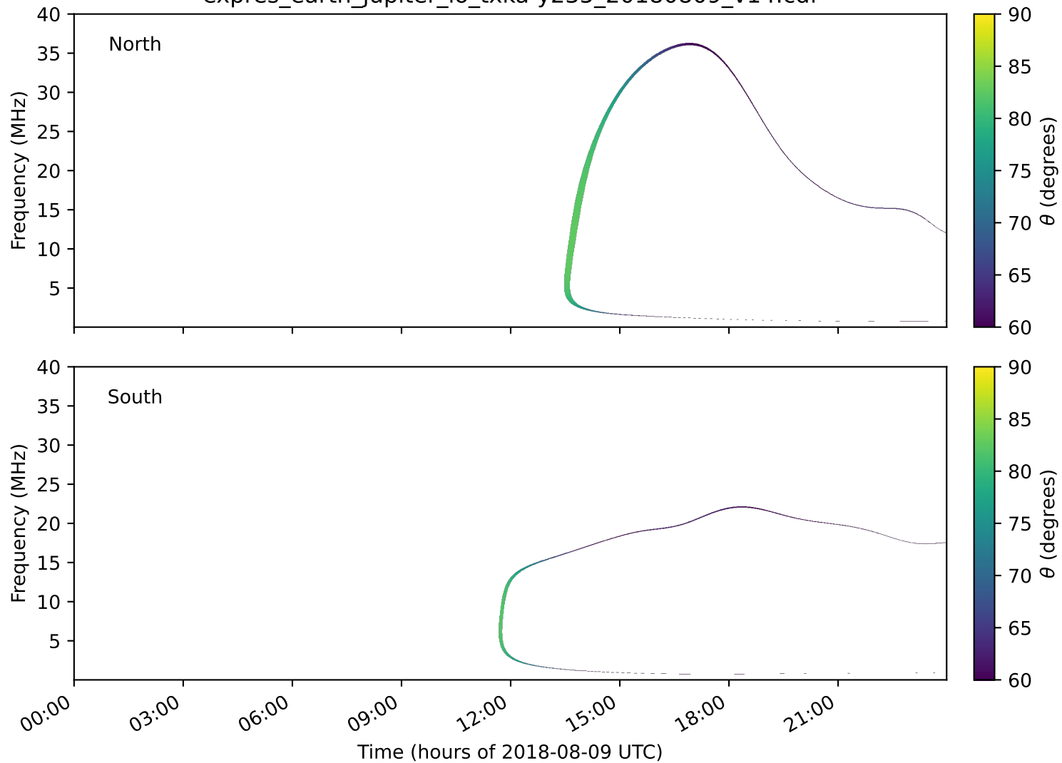
expres_earth_jupiter_io_txka-y235_20180809_v14.cdf
