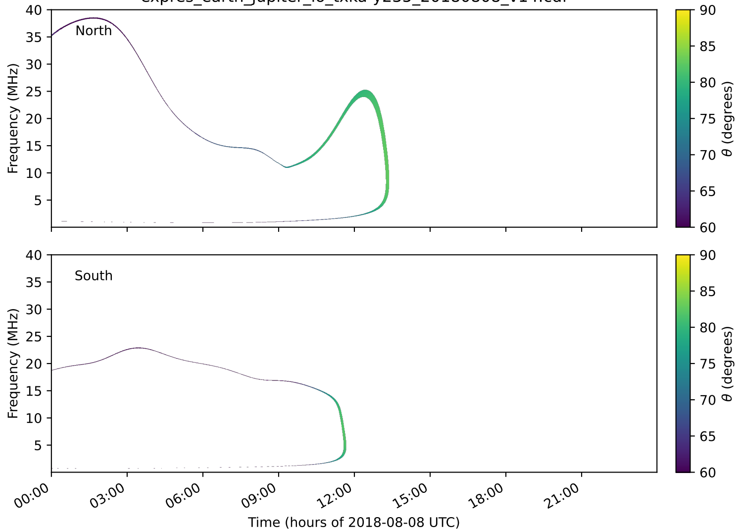
expres_earth_jupiter_io_txka-y235_20180808_v14.cdf
