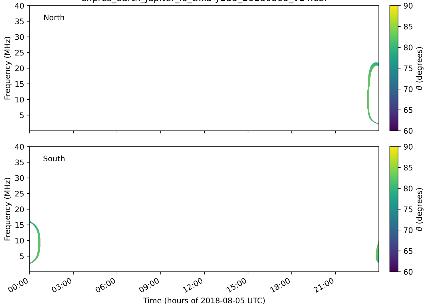
expres_earth_jupiter_io_txka-y235_20180805_v14.cdf
