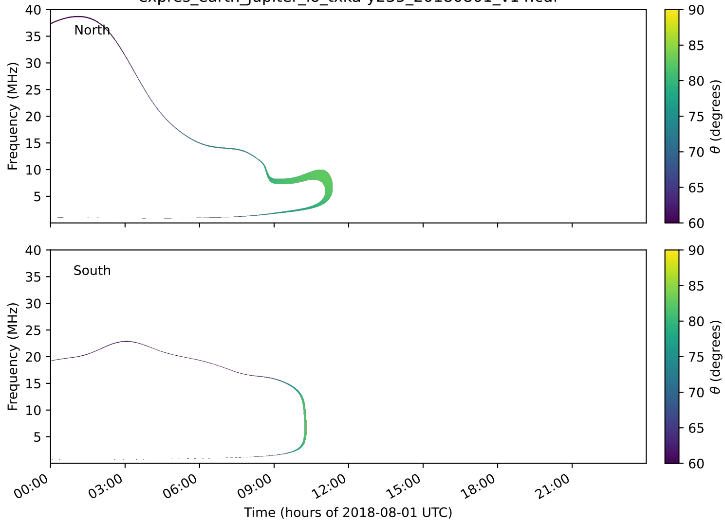
expres_earth_jupiter_io_txka-y235_20180801_v14.cdf
