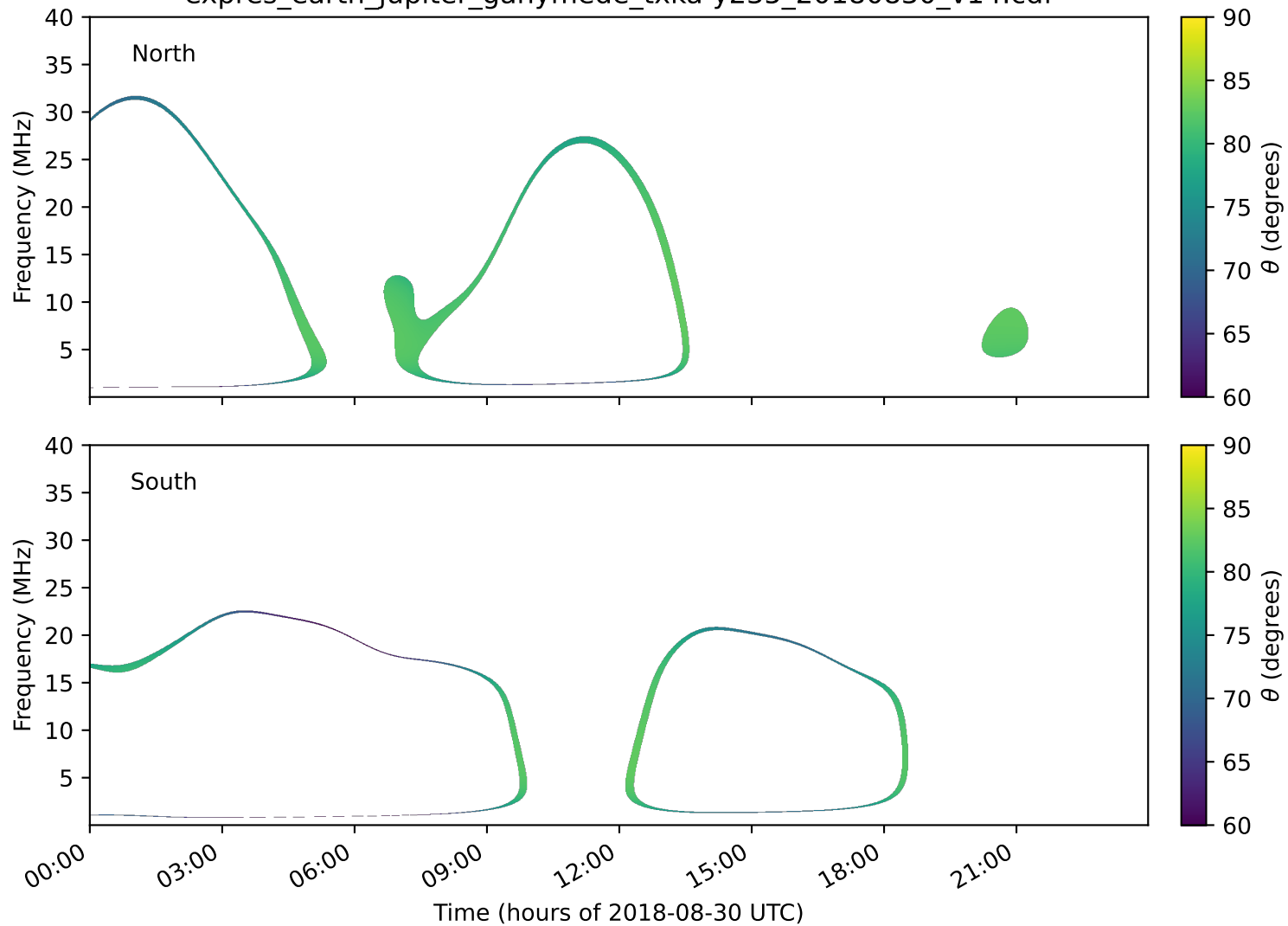
expres_earth_jupiter_ganymede_txka-y235_20180830_v14.cdf
