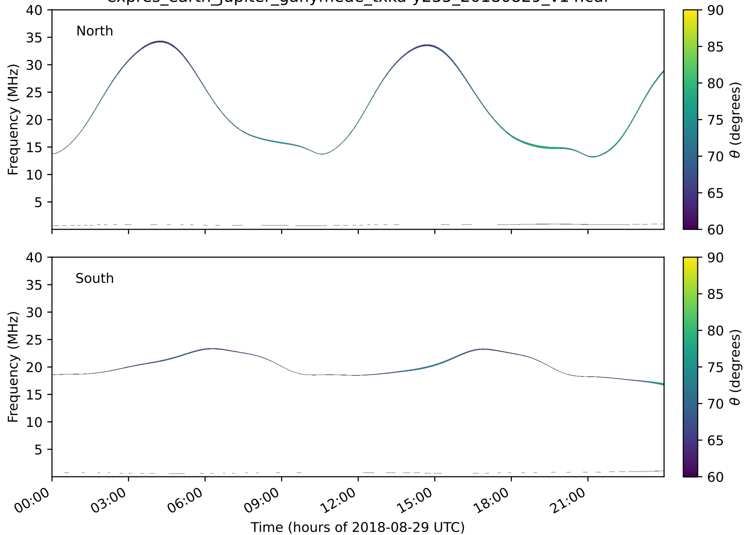
expres_earth_jupiter_ganymede_txka-y235_20180829_v14.cdf
