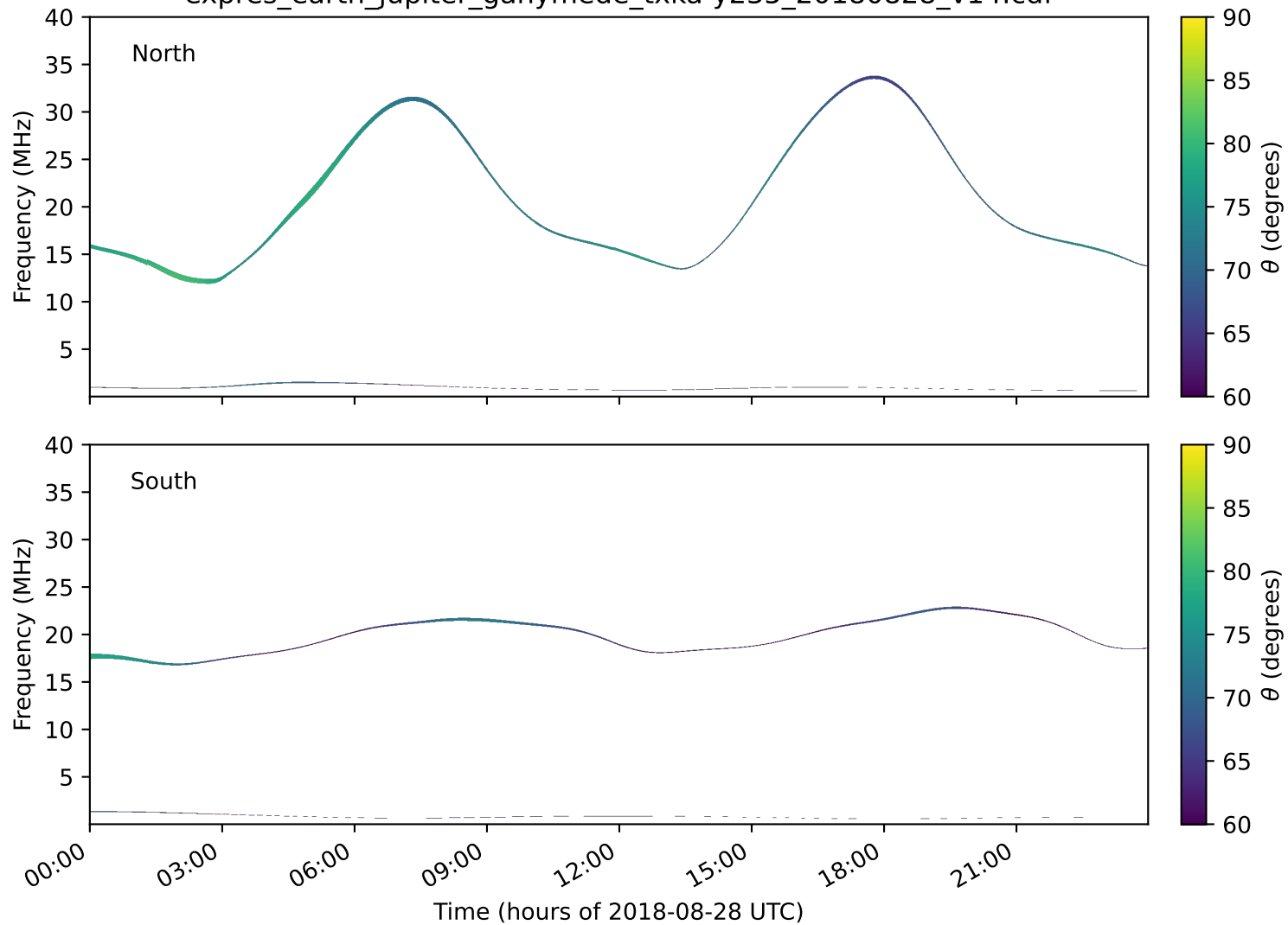
expres_earth_jupiter_ganymede_txka-y235_20180828_v14.cdf
