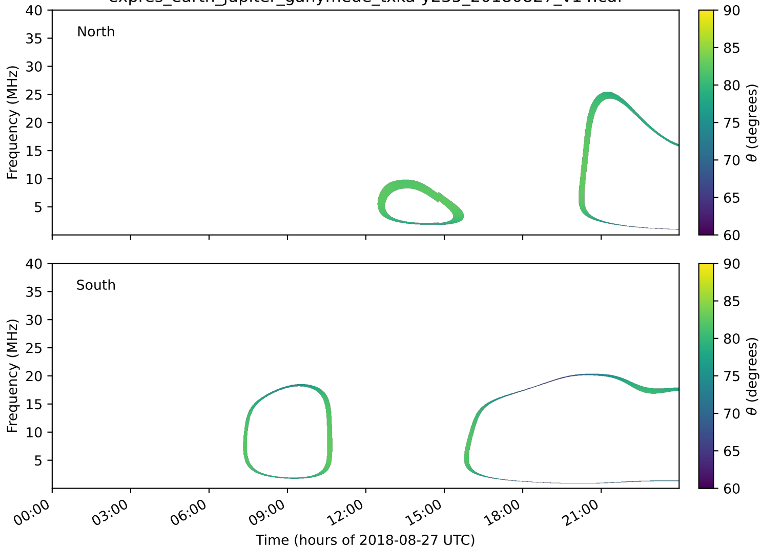
expres_earth_jupiter_ganymede_txka-y235_20180827_v14.cdf
