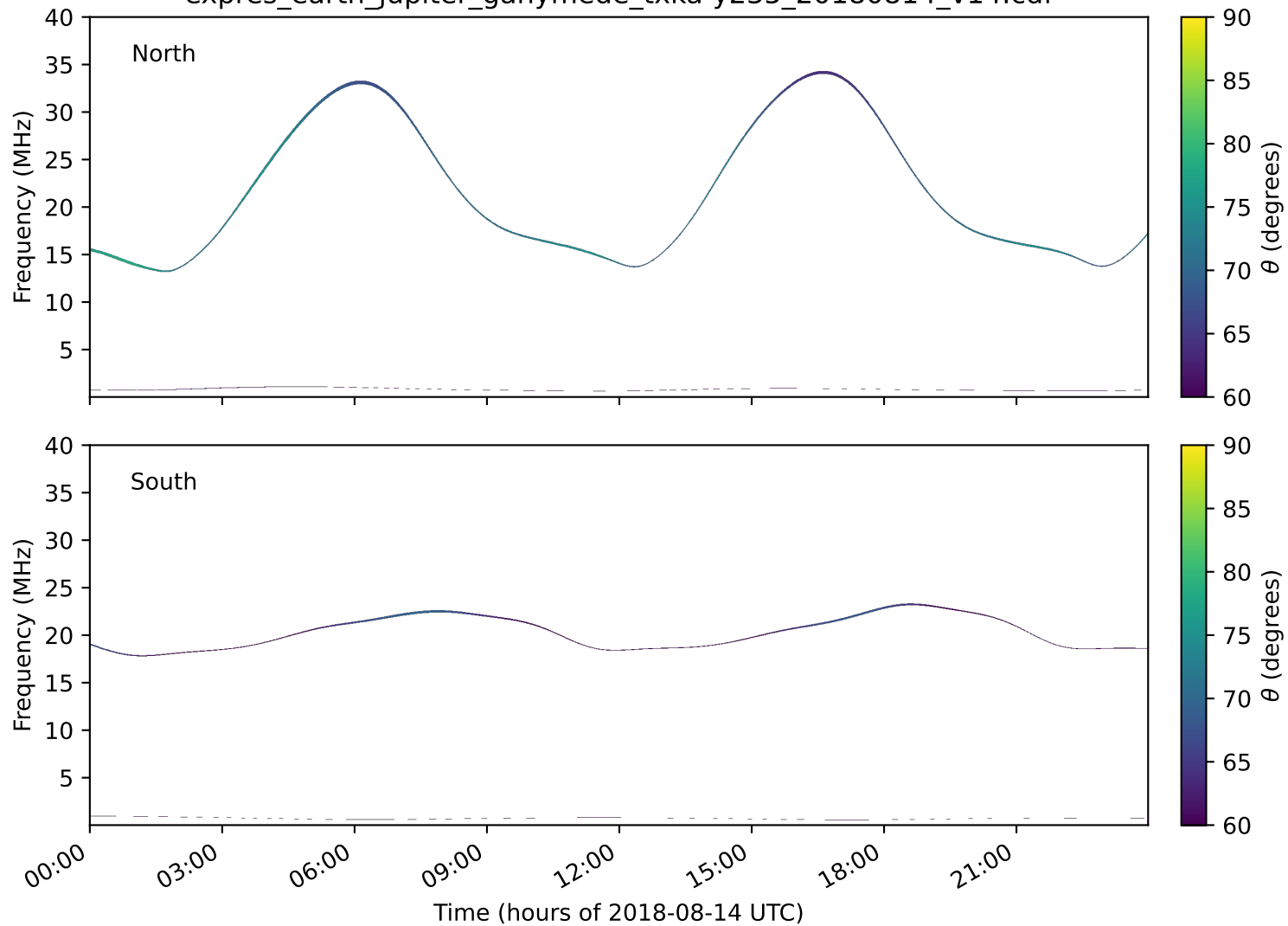
expres_earth_jupiter_ganymede_txka-y235_20180814_v14.cdf
