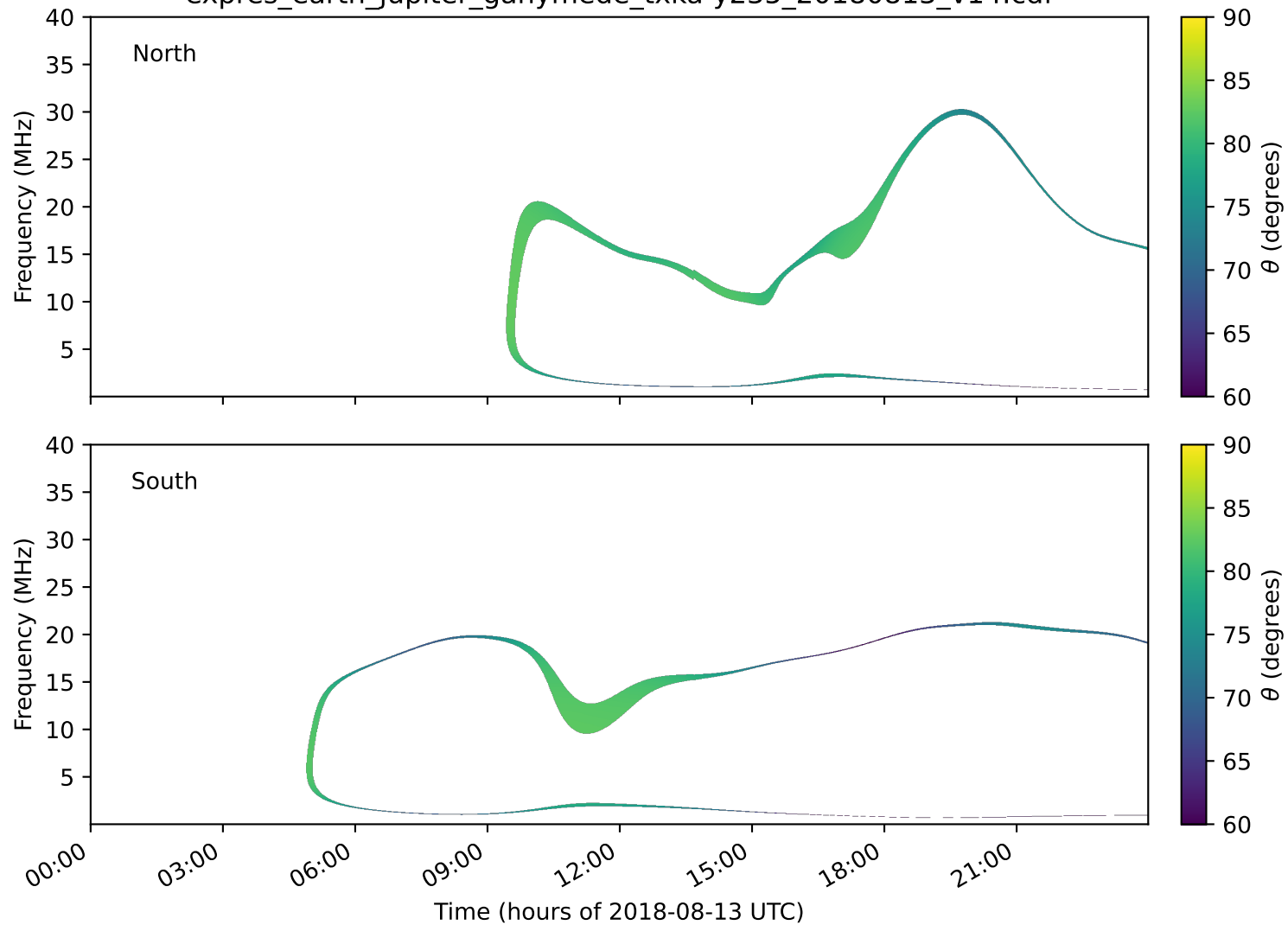
expres_earth_jupiter_ganymede_txka-y235_20180813_v14.cdf
