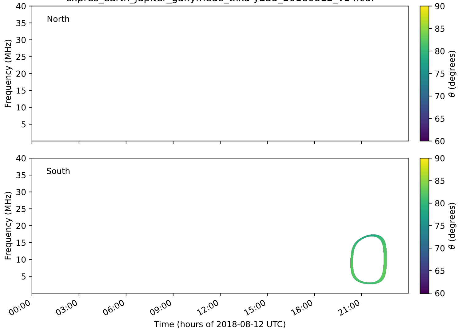
expres_earth_jupiter_ganymede_txka-y235_20180812_v14.cdf
